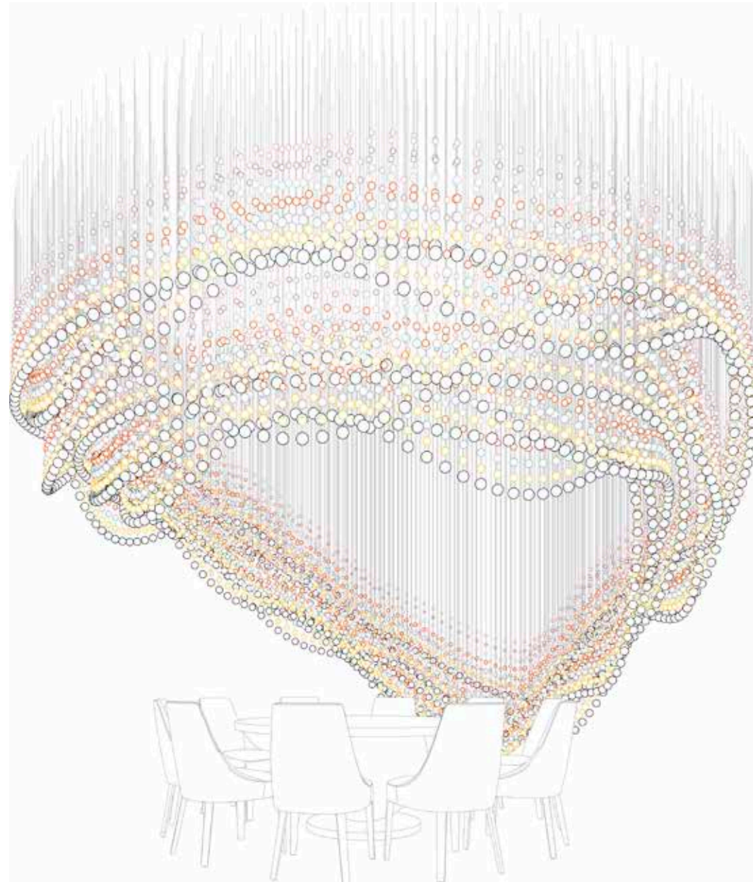
PCS01 Dimensions: 6052 • 1970 • 2863 mm Pearl Size: 20/40/50/70 mm Hanging Rope: 569 pcs
